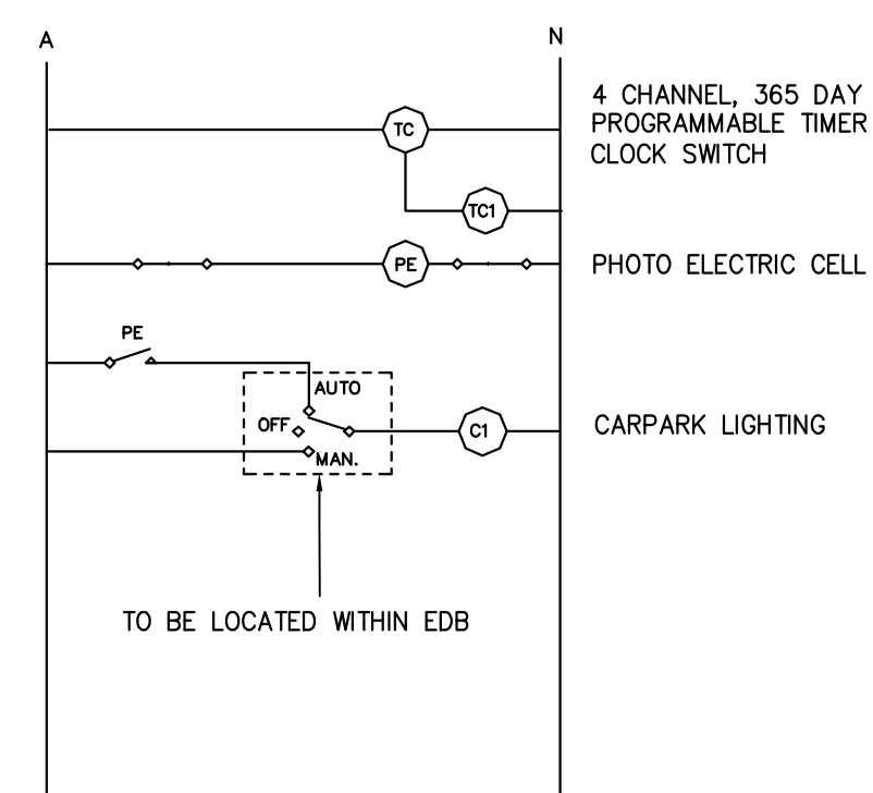
TYPICAL EXTERNAL LIGHTING CONTROL DIAGRAM
